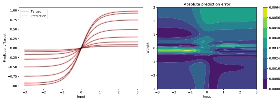
Figure B.1: We are optimizing VSML RNNs to implement neural forward computation such that for different inputs and weights a tanh-activated multiplicative interaction is produced (left), with different lines for different w . These neural dynamics are not exactly matched everywhere (right), but the error is relatively small.
