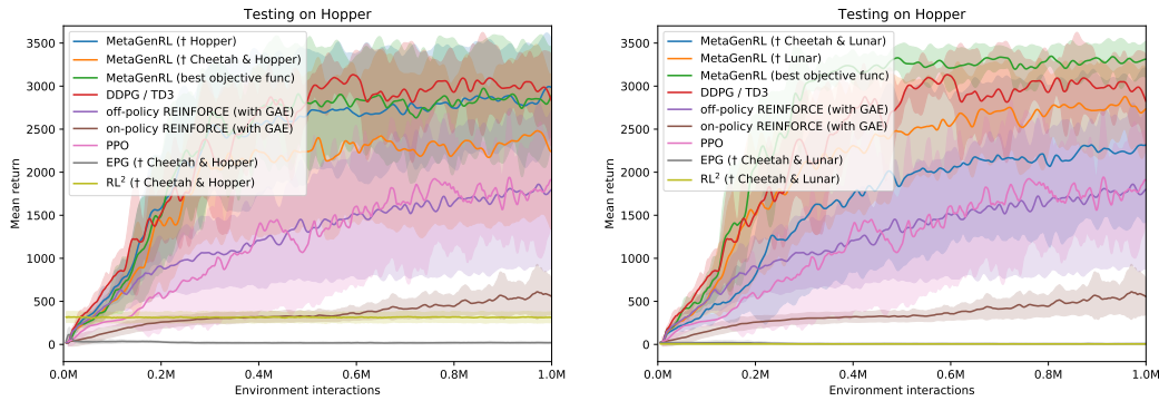
(a) Within distribution generalization.
