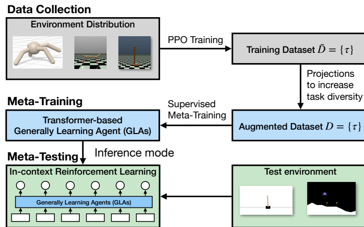
Figure 6.1: Our Generally Learning Agents (GLAs) are meta-trained on augmented RL datasets via supervised learning. First, one or more datasets of improving policies are collected using PPO. Next, these datasets are augmented with random observation and action projections to create a large diversity of tasks (environments). A Transformer is then trained to distill the (sped-up) learning process into a single in-context RL agent. Finally, at meta-test time, we can take an environment from a different domain (different actuators, observations, dynamics, and dimensionalities) and learn from rewards purely in-context without explicit hand-crafted RL algorithms or explicit gradient descent.
