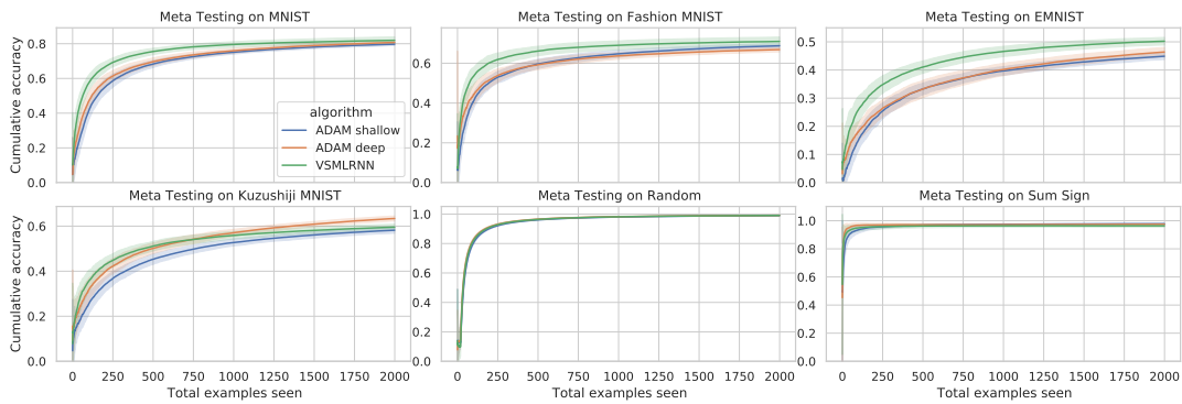
Figure B.3: Meta testing learning curves. All 6 meta test tasks are unseen. VSML RNN has been meta trained on MNIST, Fashion MNIST, EMNIST, KMNIST, and Random, excluding the respective dataset that is being meta tested on. Standard deviations are over 32 seeds.
