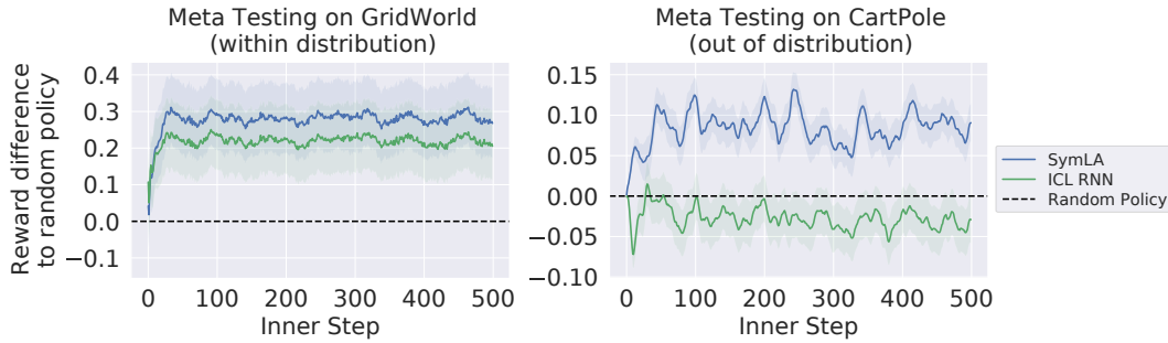
Figure 4.7: Generalisation capabilities of SymLA from GridWorld to CartPole. We meta-train the learning algorithm on GridWorld. We then meta-test on GridWorld and CartPole and report standard error of the mean and mean rewards (100 seeds) relative to a random policy - this highlights the learning process. While SymLA generalises from GridWorld to CartPole, the in-context RNN does not.
