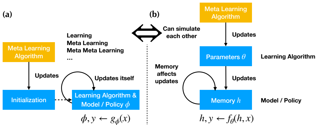
Figure 7.1: Self-referential (a) and memory-based (b) architectures (in-context learners) can represent the same function class and both require meta optimization. Self-referential networks can directly update all of their weights, whereas memory-based networks can self-modify through memory updates. The former require meta optimization of the weight initialization \phi_0 , the latter require the initial memory h_0 and weights \theta .
