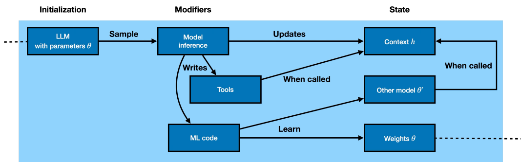
Figure 7.5: LLMs may enable various kinds of different self-referential self-improving systems.
