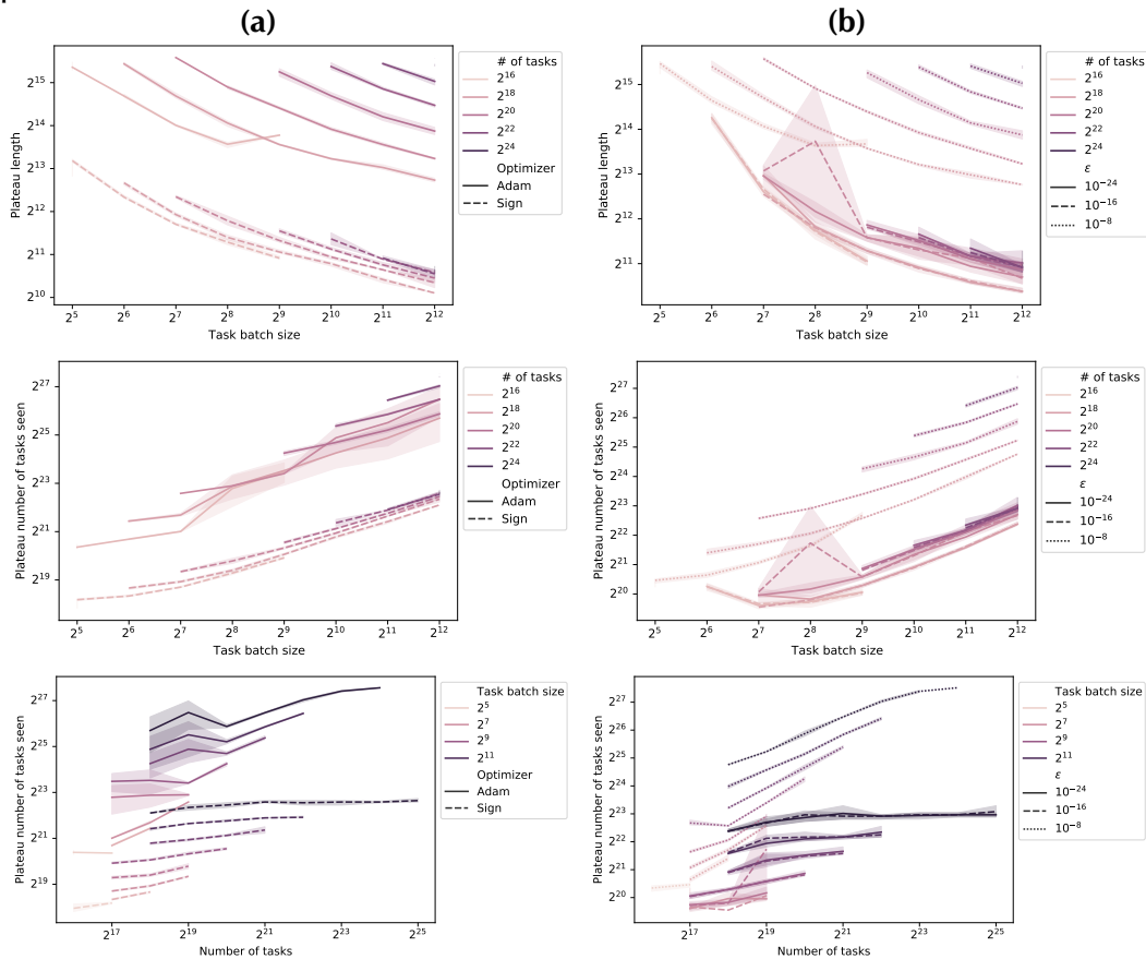
Figure D.12: (a) When replacing Adam with a sign normalization of the gradient or (b) reducing \epsilon the plateau length is significantly shorter.
