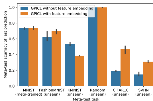
Figure 5.9: Using pre-trained networks allows leveraging domain-specific knowledge while still generalizing to other datasets GPICL is meta-trained on MNIST either with the randomly transformed raw inputs or randomly transformed pre-trained features. Pre-training helps to accelerate meta-test-time in-context learning on datasets that have a matching domain, such as CIFAR10. With only 100 examples, the learning algorithm can achieve about 45% accuracy on CIFAR10. The learning algorithms still generalize to a wide range of datasets. Error bars are 95% confidence intervals of the mean across meta-training runs.
